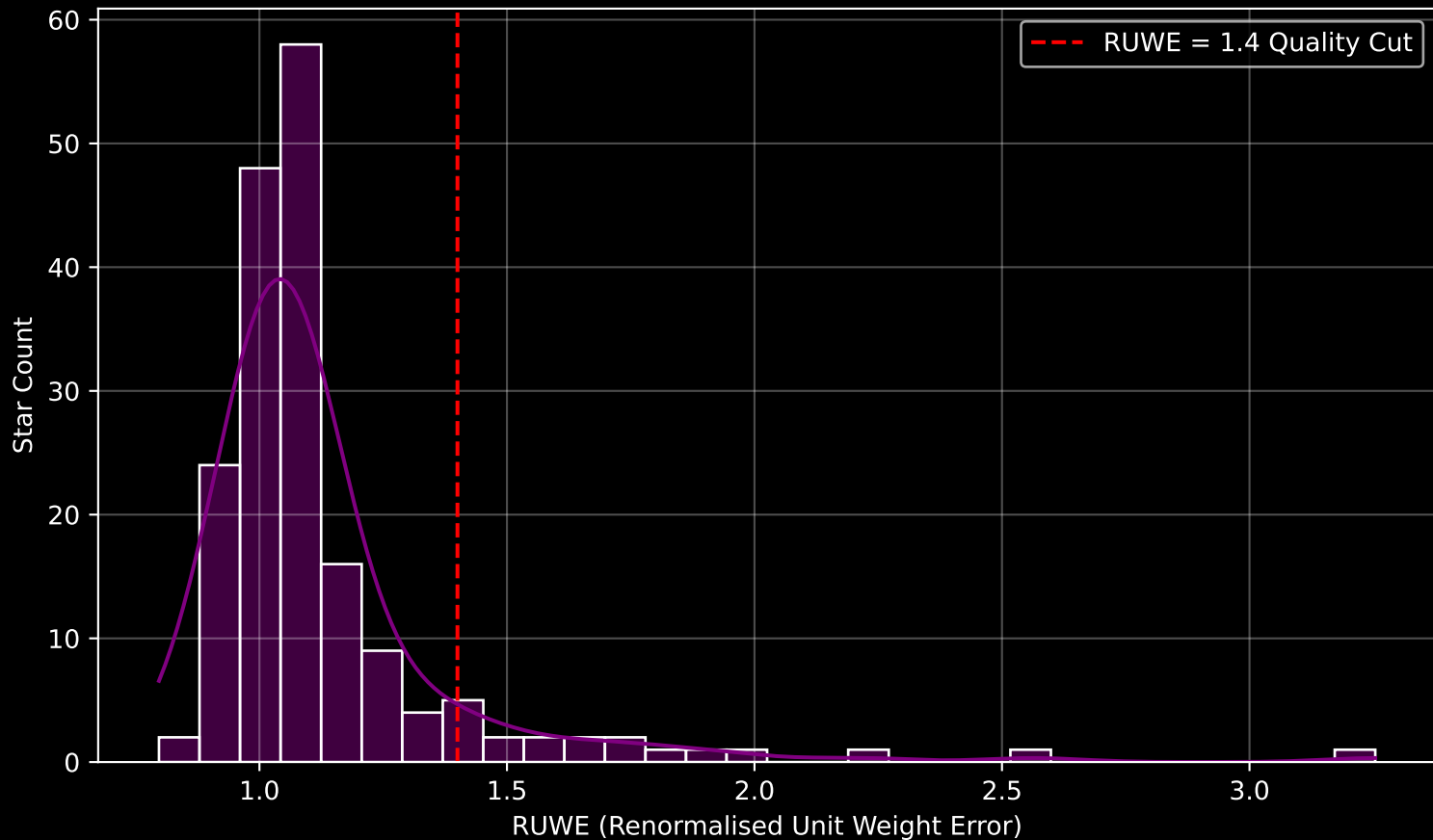
GAPOGEE DR17 Field [150-16] RUWE Distribution (n= 180)
