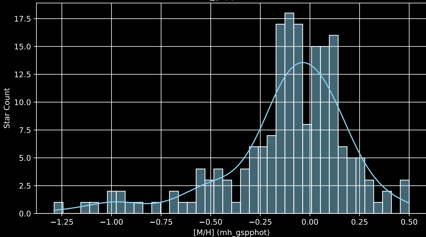
APOGEE DR17 Field: [150-16 [M/H] (mh_gspphot) (n= 183)
