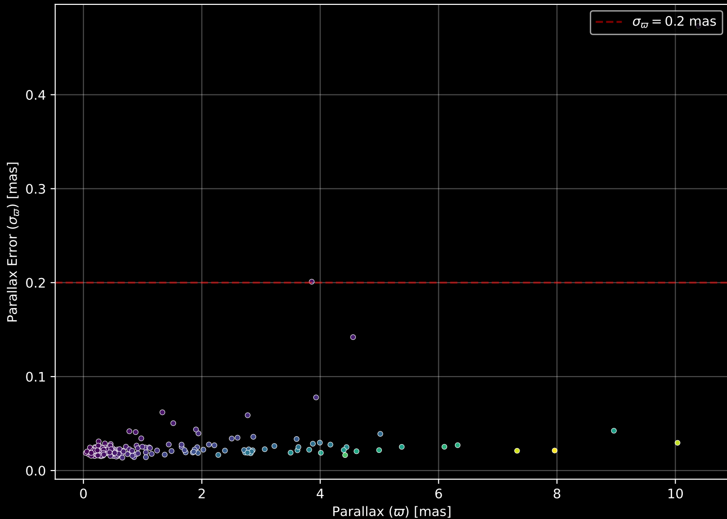
APOGEE DR17 Field: [150-16] Parallax Quality (n= 185)
