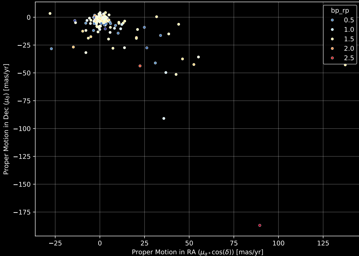
APOGEE DR17 Field: [150-16] Proper Motion Diagram (n= 185)
