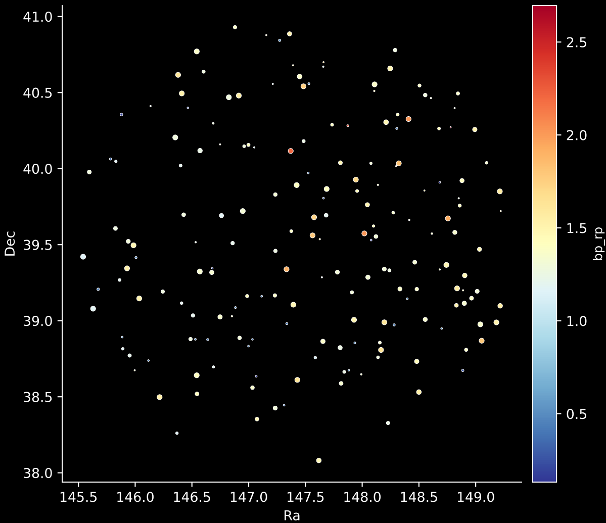
APOGEE DR17 Field: [150-16] Stars: 185
