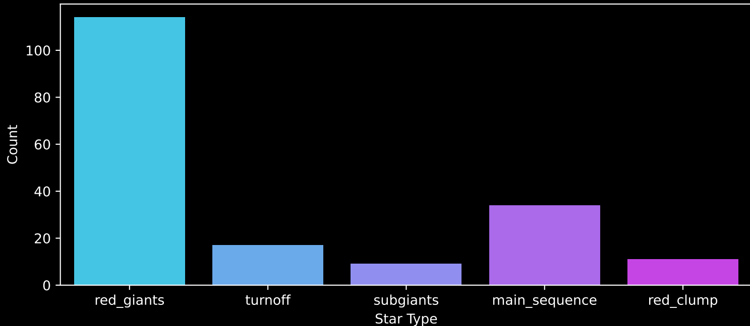
APOGEE DR17 Field: [150-16] Count plot of Star Type
